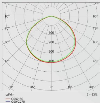
QUANG TRẮC (PHOTOMETRY)
