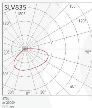
QUANG TRẮC (PHOTOMETRY)
