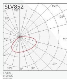
QUANG TRẮC (PHOTOMETRY)
